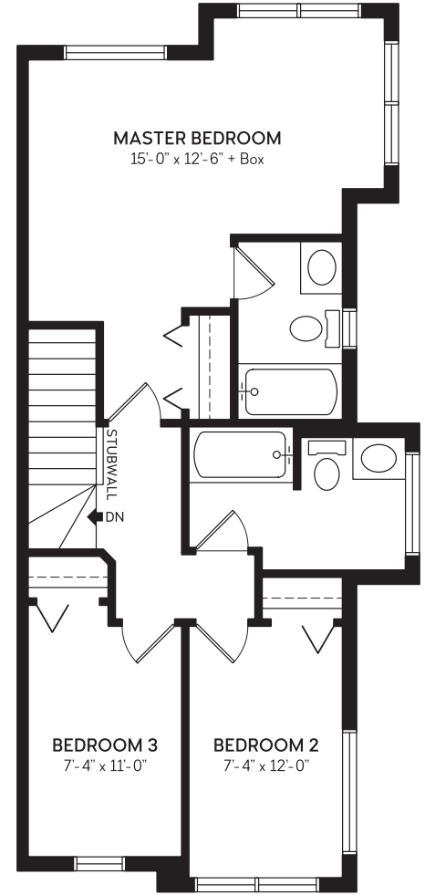
UPPER FLOOR THREE BEDROOM 668 SQ.FT.
