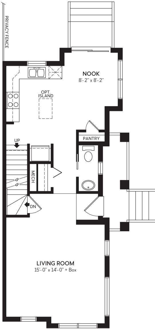
MAIN FLOOR 669 SQ.FT.
