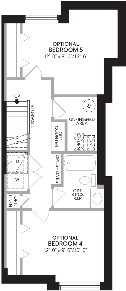
BASEMENT OPTIONAL DEVELOPMENT 485 SQ.FT.
