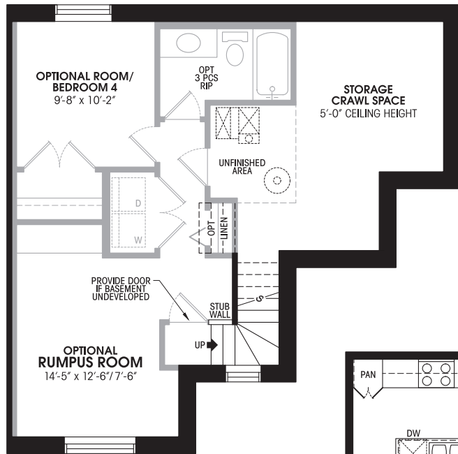
BASEMENT OPTIONAL DEVELOPMENT 433 SQ.FT.
