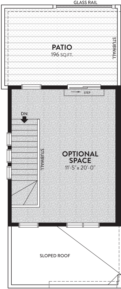
ROOFTOP 299 sq.ft.
